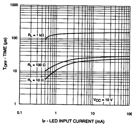
Fig. 6 Turn-Off Time vs. Input Current
